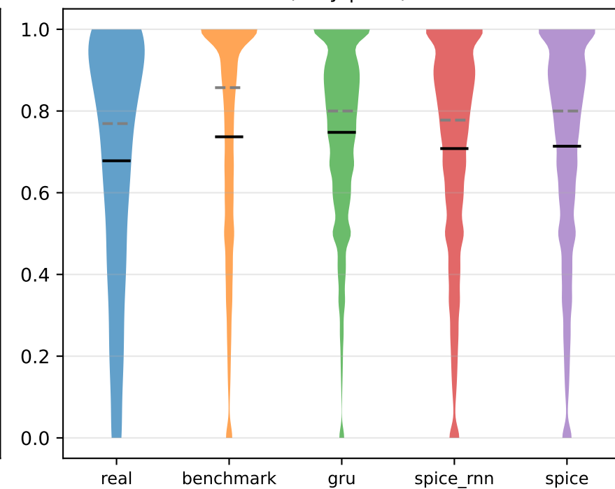
P(Stay | Win)
