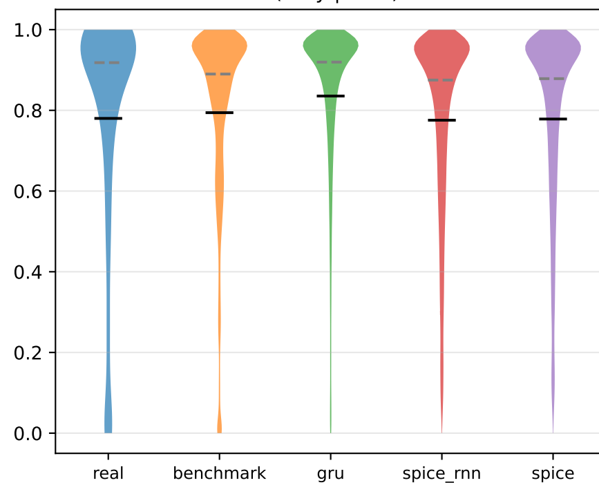
P(Stay | Loss)
