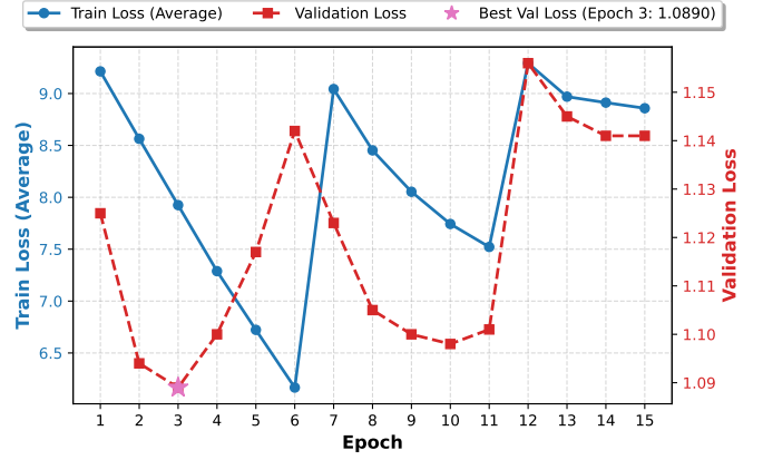
Fig. 3. Experiment 3 (Full-Scale) training and validation loss curves over 15 epochs. The left y-axis shows the average training loss (blue circle), while the right y-axis displays the validation loss (red square). The star marker highlights the optimal generalization checkpoint at Epoch 3 (1.0890).
