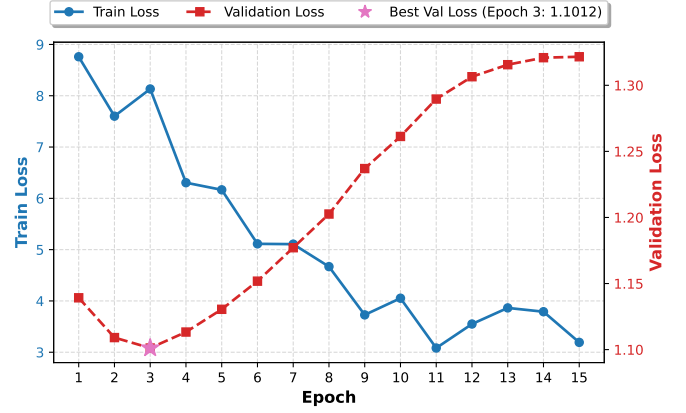
Fig. 1. Experiment 1 (Pilot Study) training and validation loss curves over 15 epochs. The left y-axis shows the training loss (blue circle), while the right y-axis displays the validation loss (red square). The star marker highlights the optimal generalization checkpoint at Epoch 3 (1.1012).
