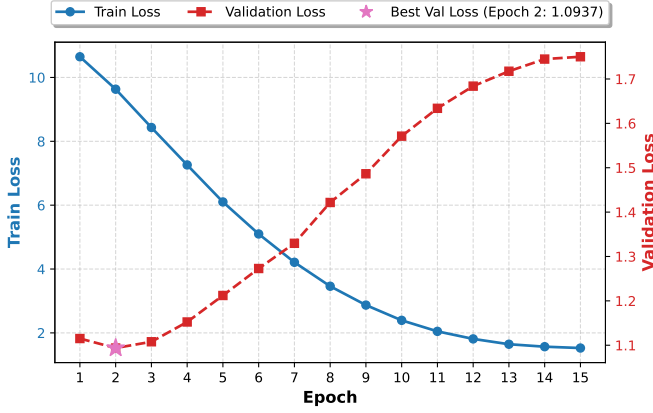
Fig. 2. Experiment 2 (Data Augmentation) training and validation loss curves over 15 epochs. The left y-axis shows the average training loss (blue circle), while the right y-axis displays the validation loss (red square). The star marker highlights the optimal generalization checkpoint at Epoch 2 (1.0937).
