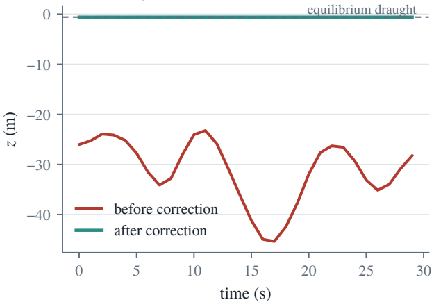
(a) hull height
