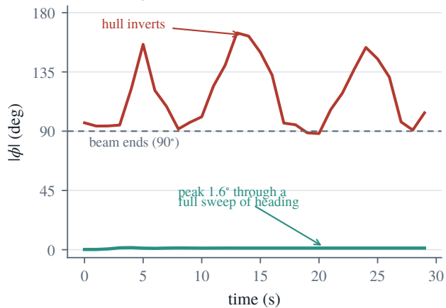
(b) roll angle
