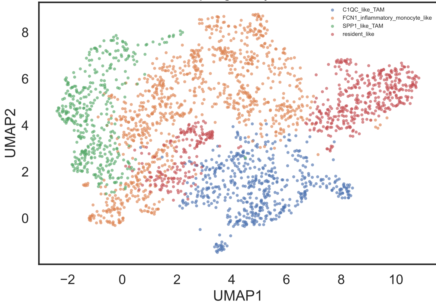
Macrophage-only UMAP
