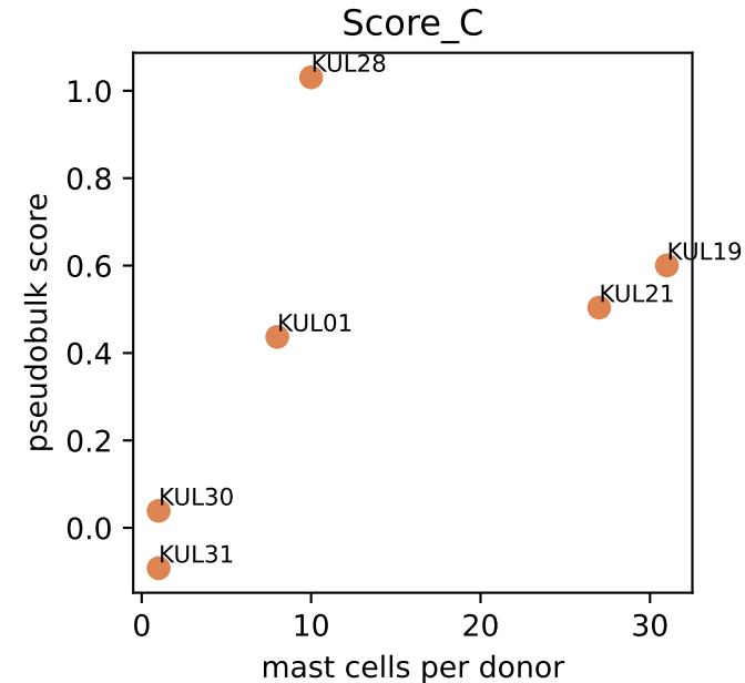
Mast-cell count versus PGE2 score
