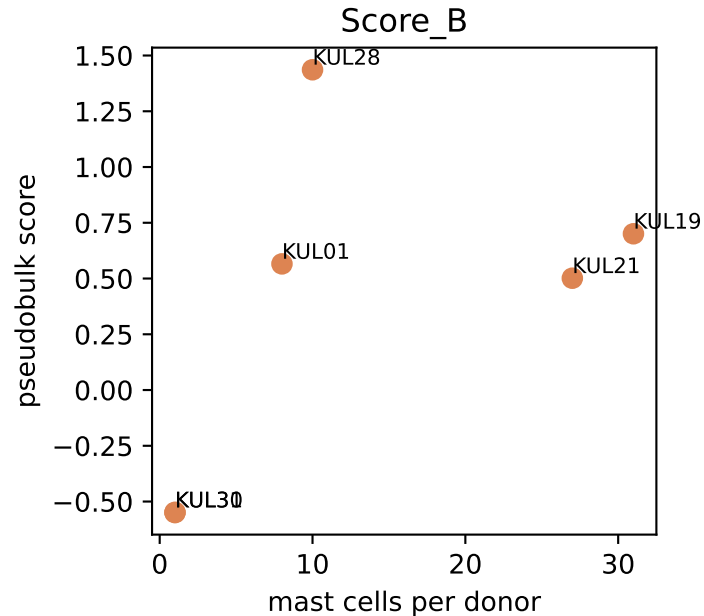
Mast-cell count versus PGE2 score
