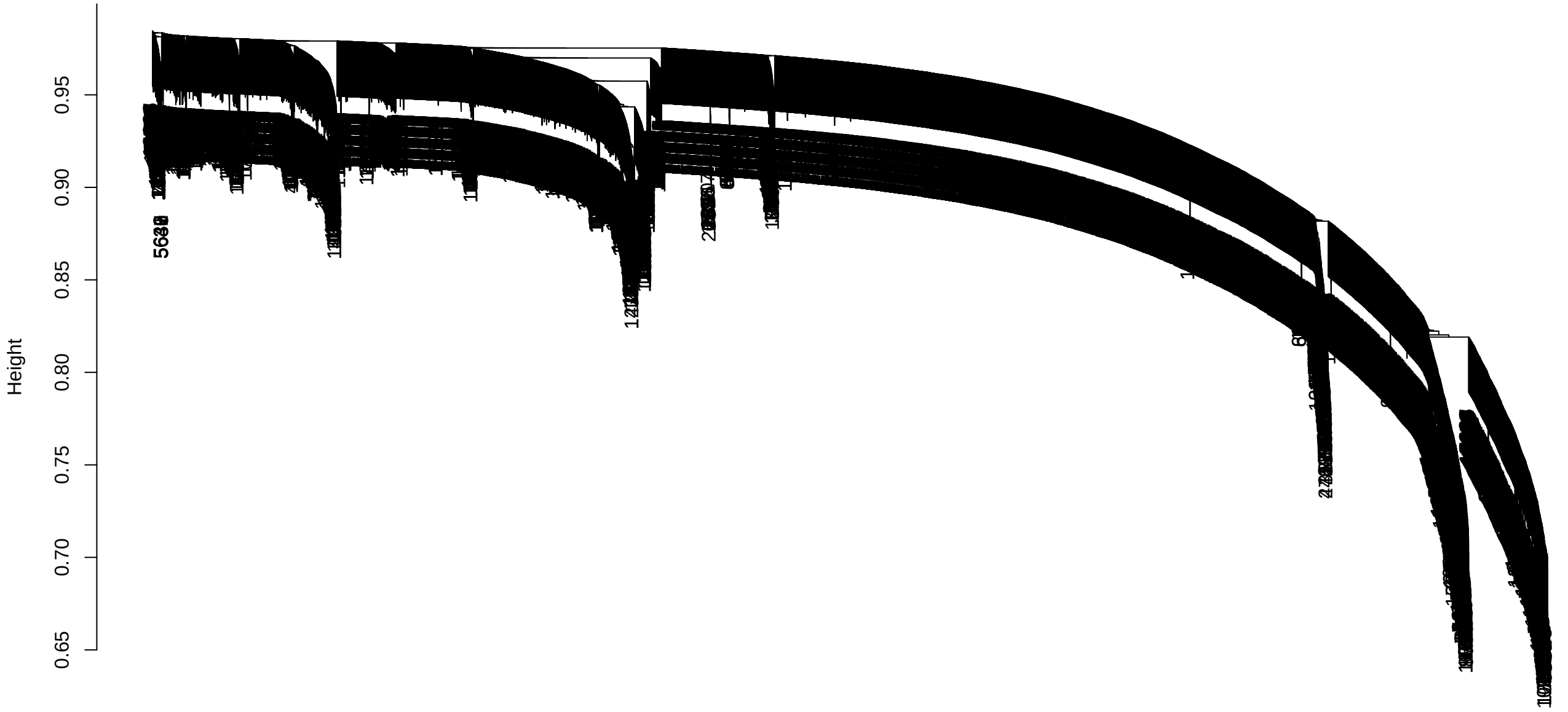
WGCNA gene dendrogram, block 1
