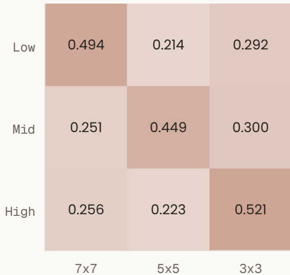
Mean sparse mixing weight
