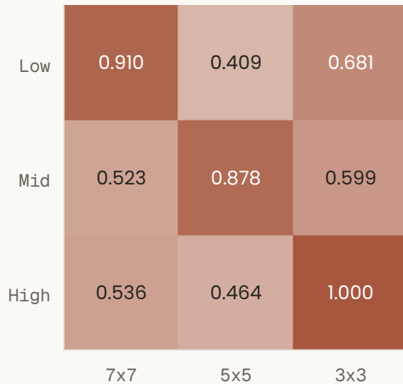
Fraction of pixels selecting expert
