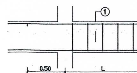
LONG SECTION
