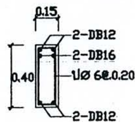
SECTION 1-1
