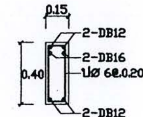
SECTION 1-1
