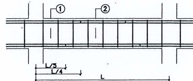
LONG SECTION
