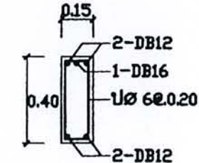
SECTION 1-1
