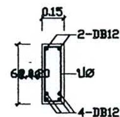
SECTION 2-2
