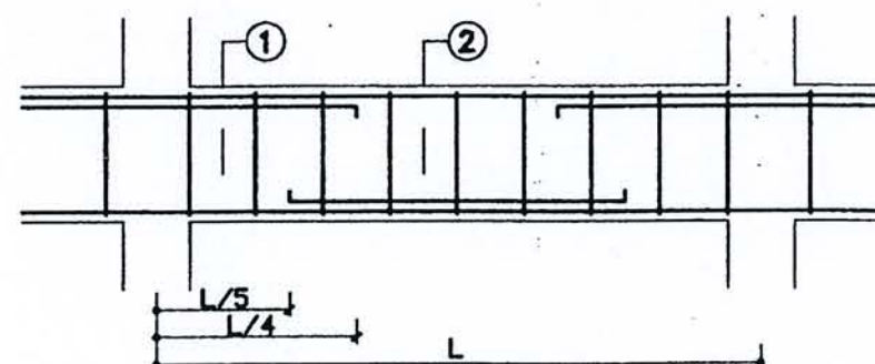
LONG SECTION
