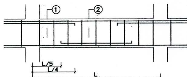
LONG SECTION
