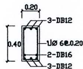
SECTION 2-2
