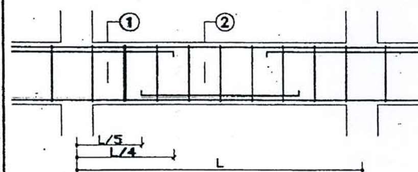
LONG SECTION
