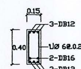
SECTION 2-2
