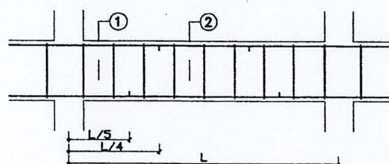
LONG SECTION
