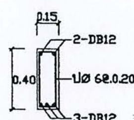
SECTION 2-2
