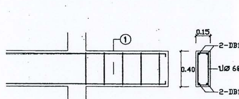
LONG SECTION
