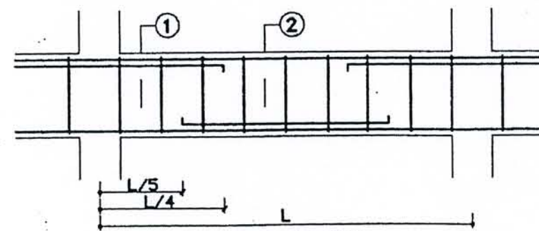
LONG SECTION
