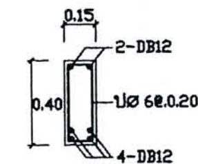
SECTION 2-2
