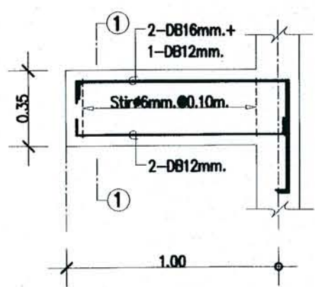
LONG SECTION BC
