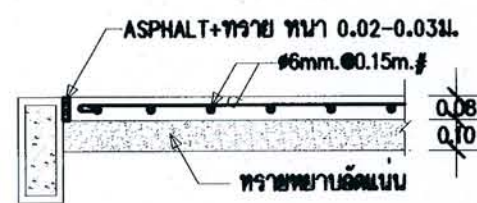
DETAIL SO
