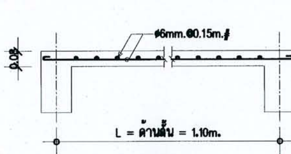
DETAIL S1
