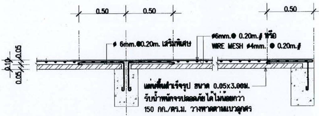
DETAIL SP
