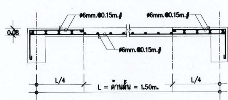
DETAIL S2
