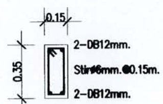
DETAIL BS=B2
