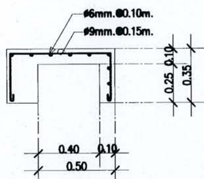
DETAIL SC
