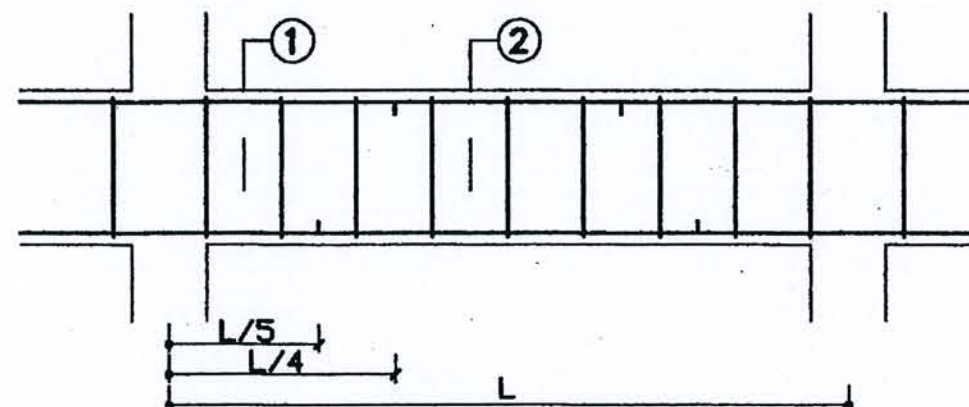
LONG SECTION
