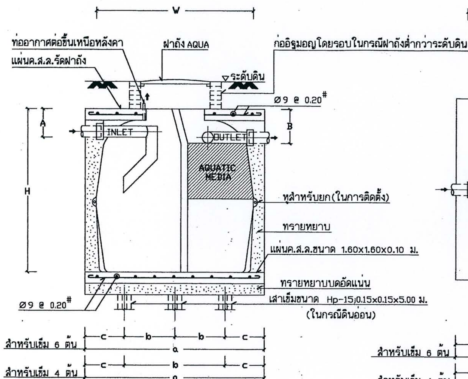
SECTION 1:20
