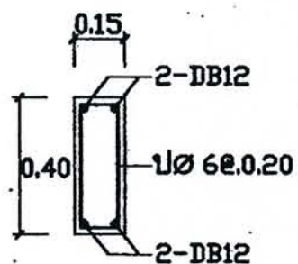
SECTION 1-1
