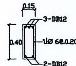
SECTION 1-1
