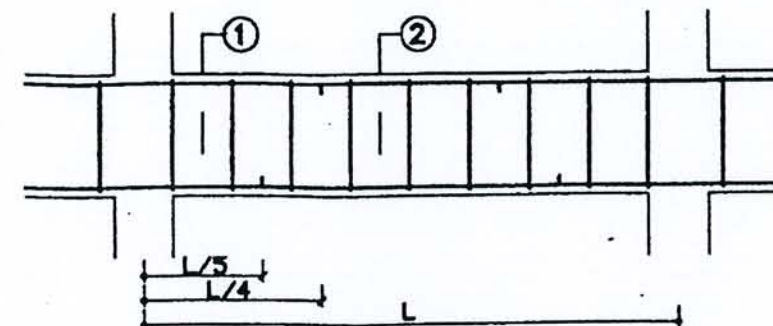
LONG SECTION
