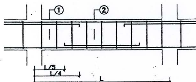
LONG SECTION
