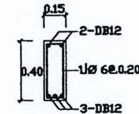
SECTION 2-2
