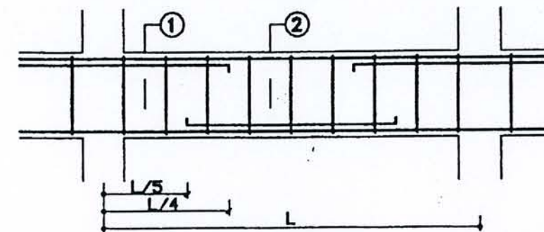
LONG SECTION
