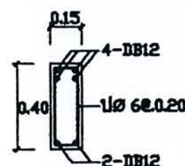
SECTION 1-1
