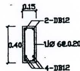
SECTION 2-2
