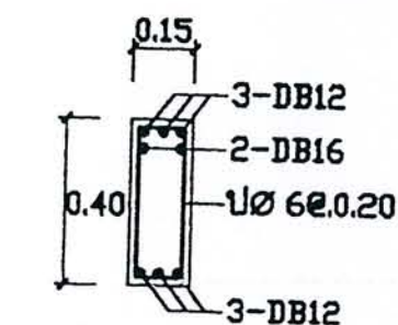
SECTION 1-1
