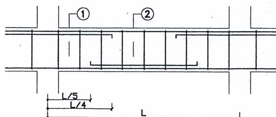
LONG SECTION
