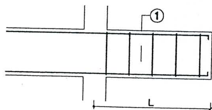
LONG SECTION
