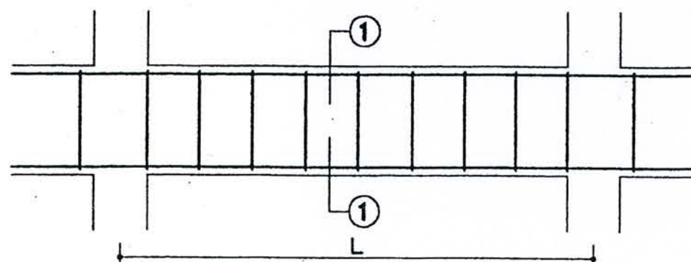
LONG SECTION
