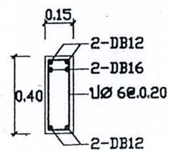
SECTION 1-1
