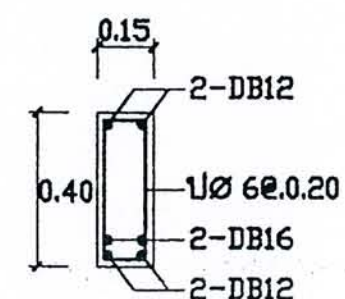
SECTION 2-2
