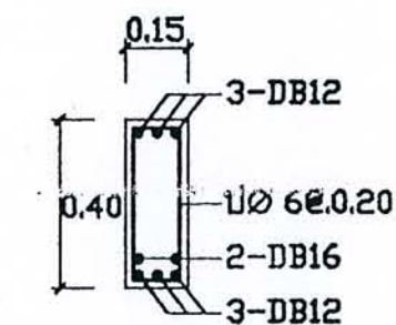
SECTION 2-2
