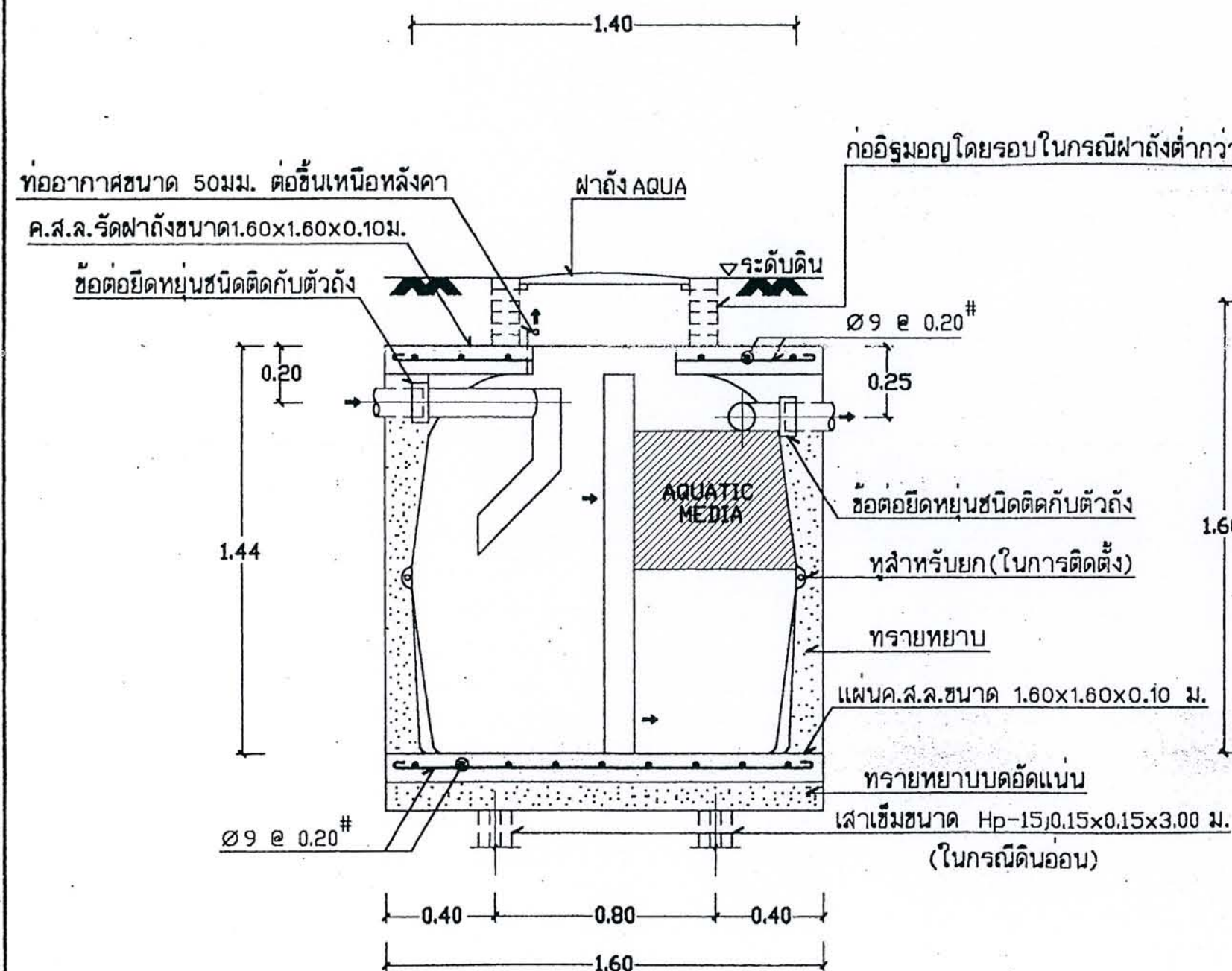
SECTION 1:20
