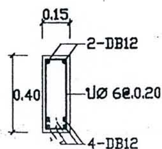
SECTION 2-2
