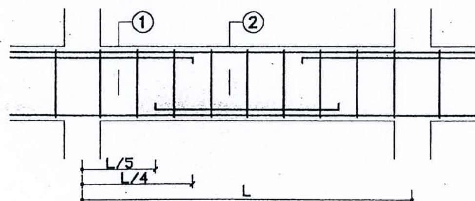
LONG SECTION
