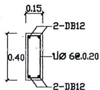
SECTION 1-1
