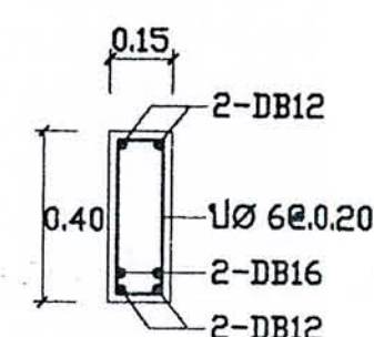
SECTION 2-2
