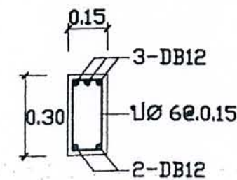
SECTION 1-1
