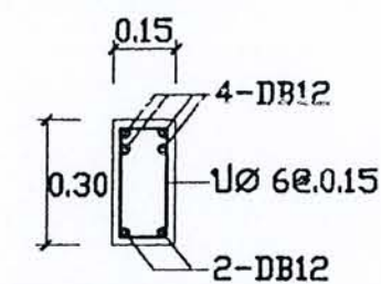
SECTION 1-1
