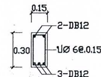
SECTION 2-2
