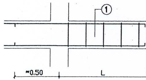
LONG SECTION
