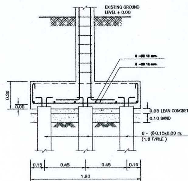
FOOTING "F2" SCALE 1:25
