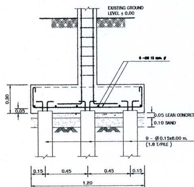
FOOTING "F1" SCALE 1:25
