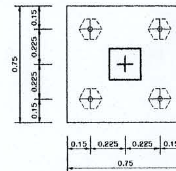
PLAN SCALE 1:25
