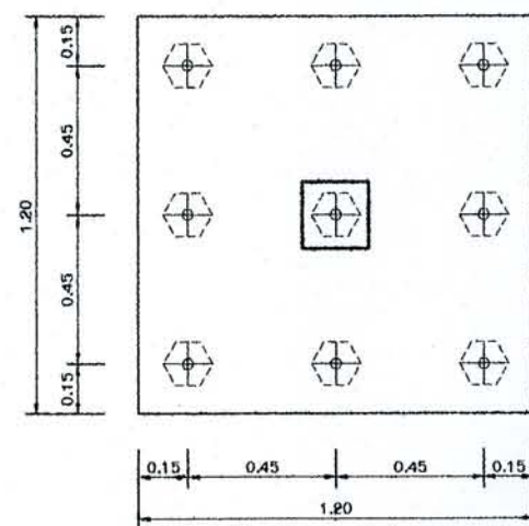
PLAN SCALE 1:25
