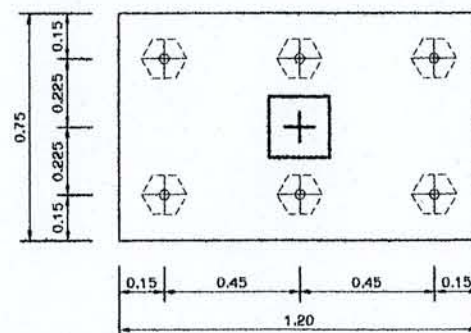
PLAN SCALE 1:25
