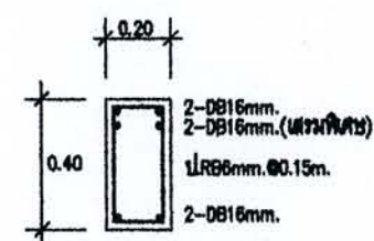
B12A ②-② 1:25
