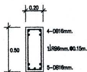
B8 1:25
