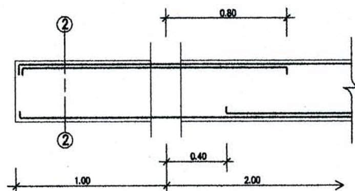
B12A
