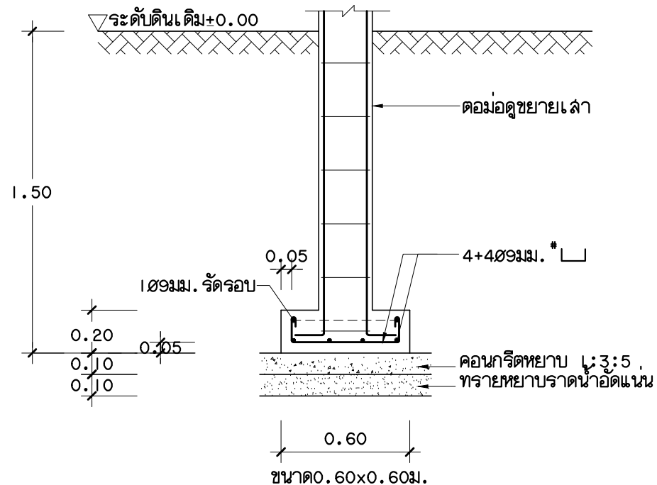
F0.60x0.60 1:25
