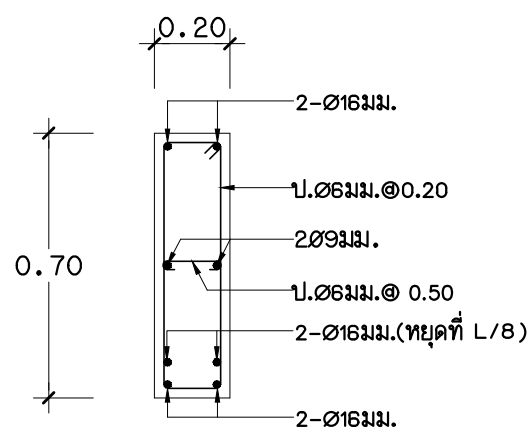
B4A 1:20
