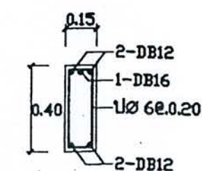
SECTION 1-1
