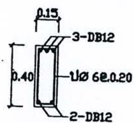
SECTION 1-1
