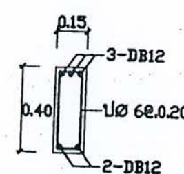
SECTION 1-1
