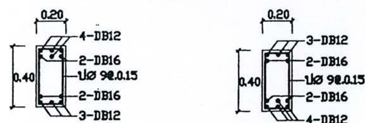
SECTION 1-1
