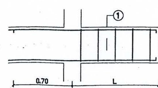
LONG SECTION
