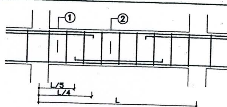
LONG SECTION
