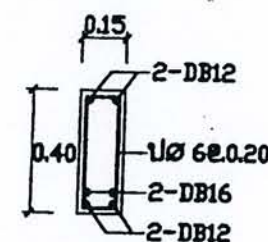
SECTION 2-2
