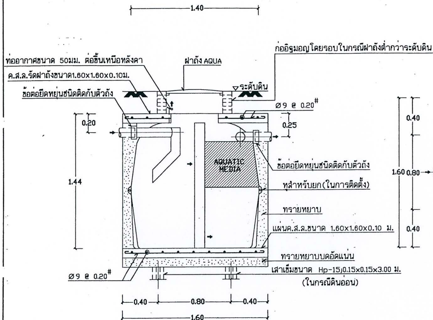
SECTION 1:20
