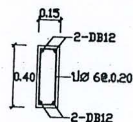
SECTION 1-1
