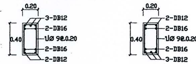
SECTION 1-1
