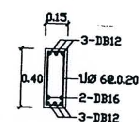
SECTION 2-2
