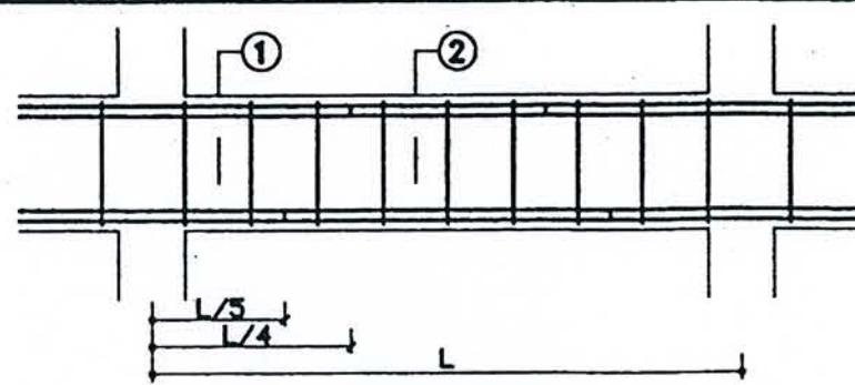
LONG SECTION
