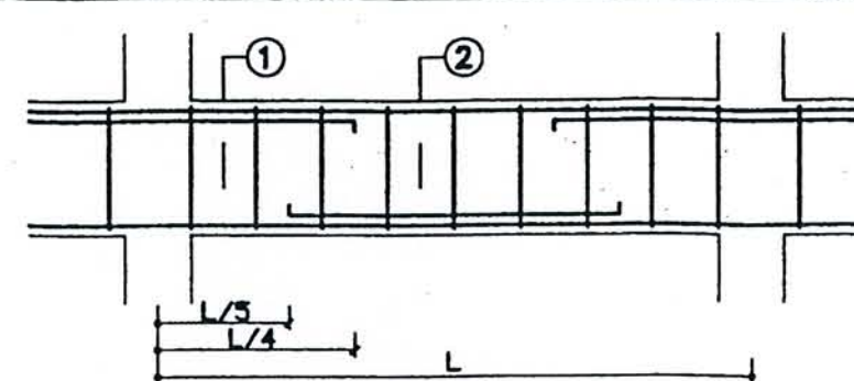
LONG SECTION
