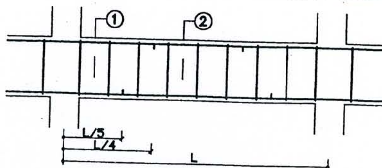
LONG SECTION
