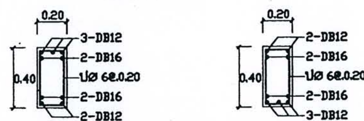
SECTION 1-1
