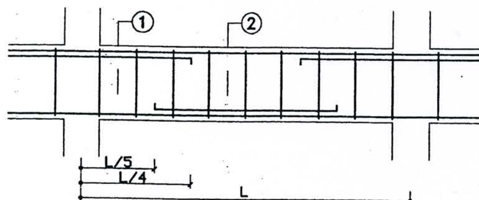
LONG SECTION
