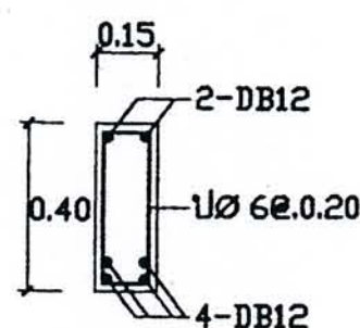
SECTION 2-2
