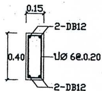
SECTION 1-1
