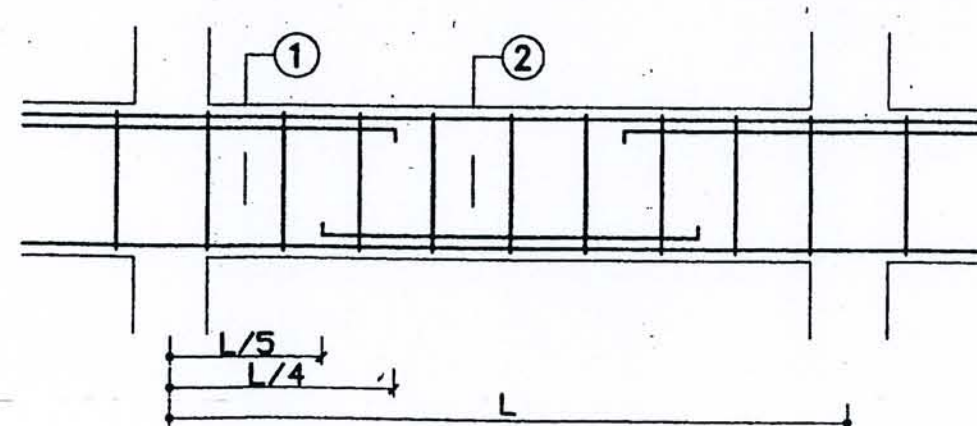
LONG SECTION
