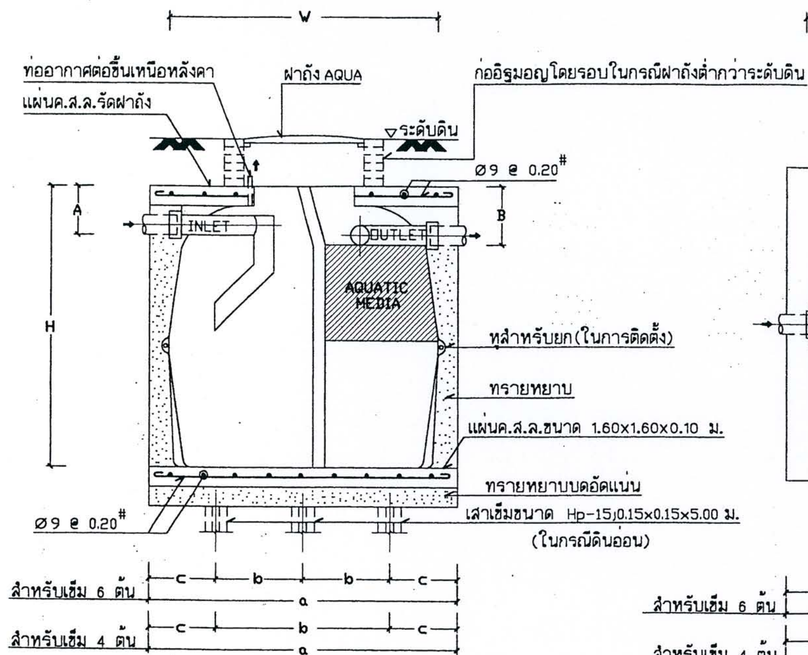
SECTION 1:20
