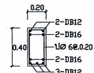
SECTION 2-2
