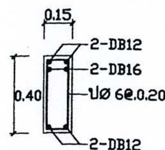
SECTION 1-1
