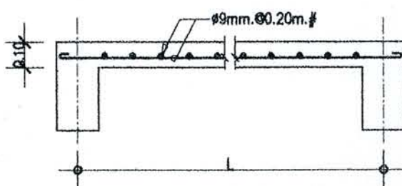
DETAIL S1
