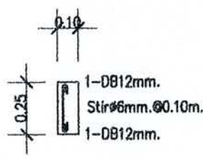
SECTION 1-1 (BO)
