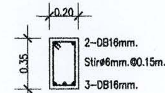
DETAIL B4
