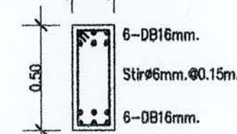
DETAIL B8
