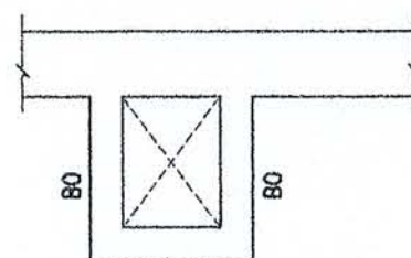
DETAIL DUCT
