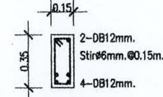
DETAIL B2
