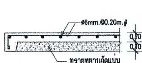
DETAIL GS
