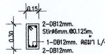
DETAIL B9
