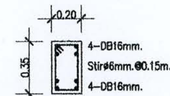
DETAIL B6
