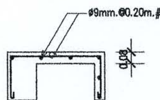
DETAIL CS
