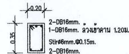
DETAIL CB3
