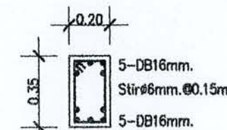
DETAIL B7
