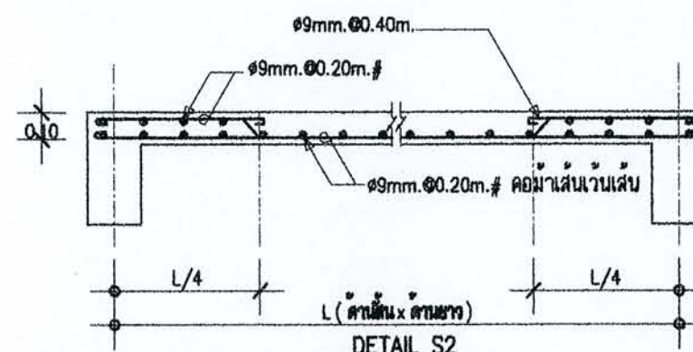
DETAIL S2
