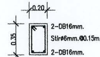
DETAIL B3
