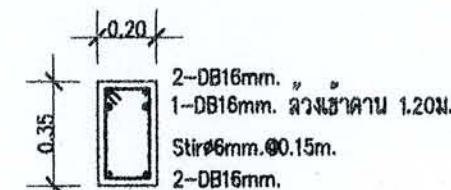
DETAIL CB5
