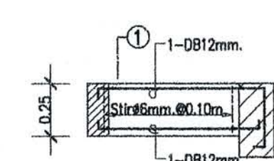
LONG SECTION BO
