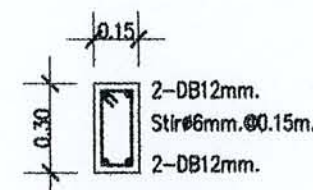
DETAIL B1
