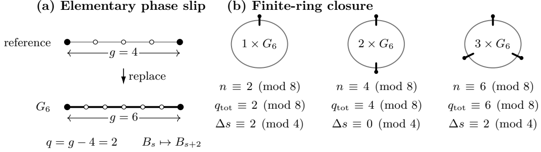
Figure 2: Reference gaps and charge-compatible phase slips. A G_6 replaces g = 4, q = 0 by g = 6, q = 2 ; one, two, and three copies provide the mod-eight total charges for residues 2, 4, 6, while their mod-four sector transport is checked independently.
