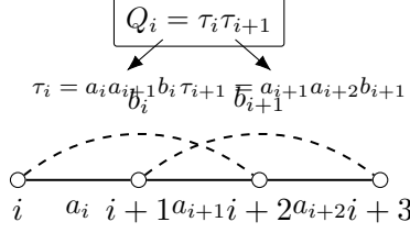
Figure 1: Local flux coordinates in C_n(1, 2) . Solid edges have cyclic distance one and dashed arcs have distance two. The adjacent triangle fluxes share the edge sign a_{i+1} ; their product is the quadrilateral flux Q_i . The drawing fixes notation only and does not impose a gauge.
