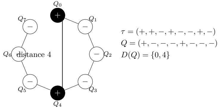
Figure 2: The target period-eight phase. The triangle-flux word \tau induces the quadrilateral-flux word Q with exactly two positive entries, shown as filled vertices. They are antipodal in the eight-site cell, so D(Q) = \{0, 4\} up to translation and reflection. This geometry is the sub-eight case isolated by the trichotomy in Section 6.
