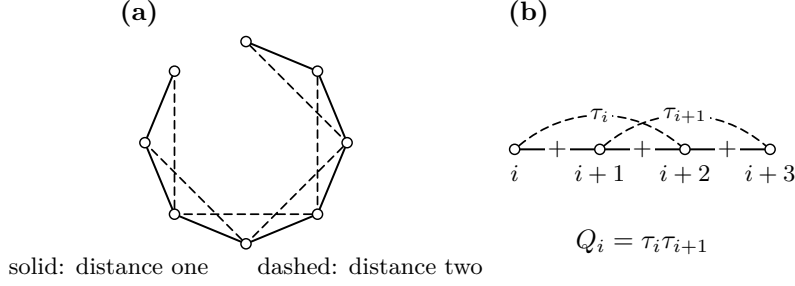
Figure 1: The cycle square and Hamilton-gauge coordinates.
