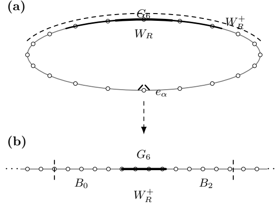
Figure 4: Identification of a finite localization patch with the bilateral G6 model.
