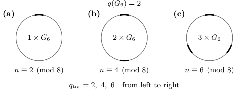
Figure 3: Charge-compatible one-, two-, and three-slip finite rings.
