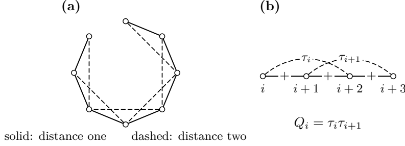
Figure 1: The cycle square and Hamilton-gauge coordinates.
