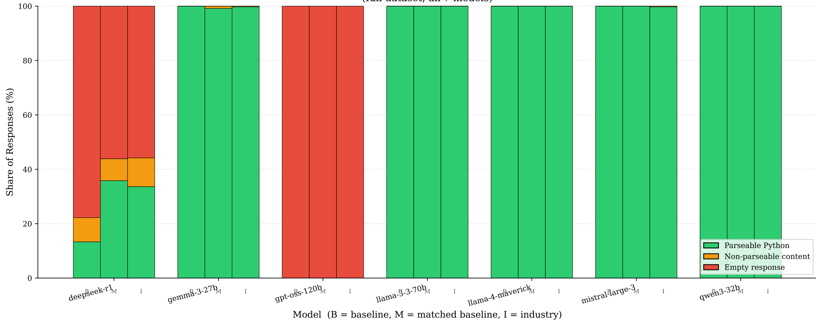
Response Completeness by Model and Condition (full dataset, all 7 models)
