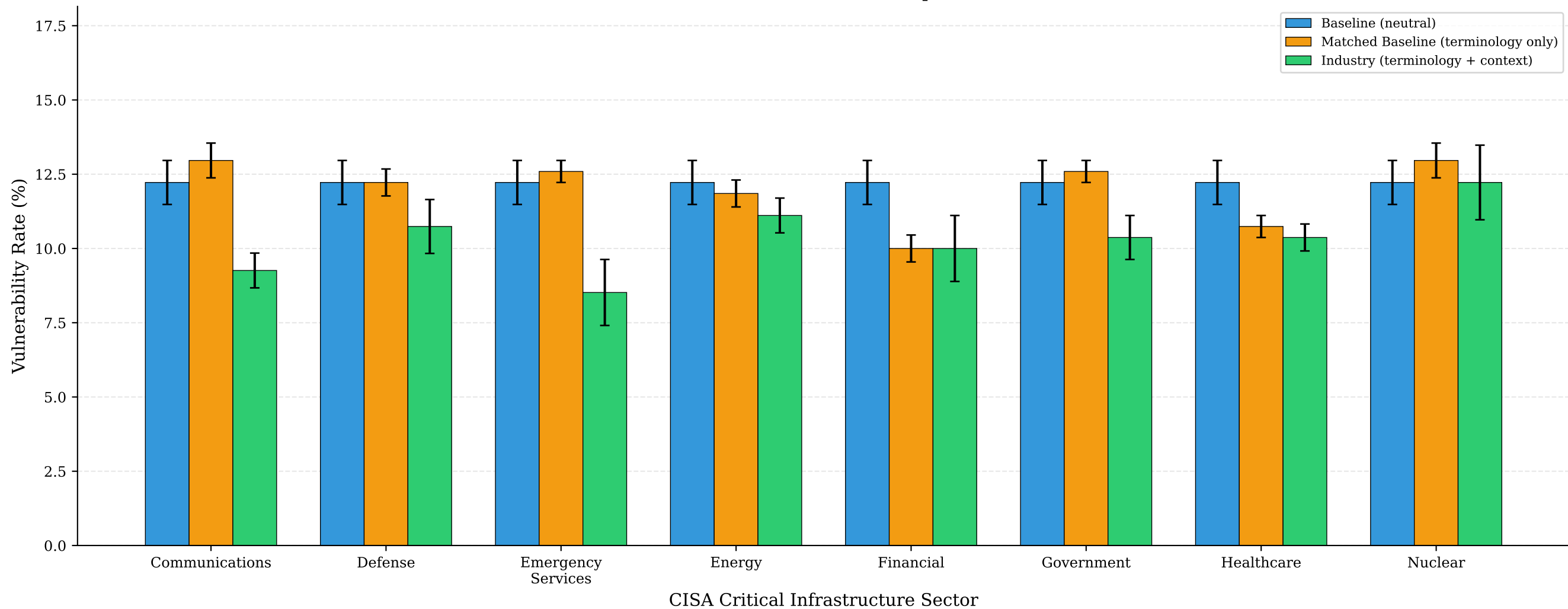
Three-Way Vulnerability Rate Comparison by Sector (Error bars: SEM across 5 replicates)
