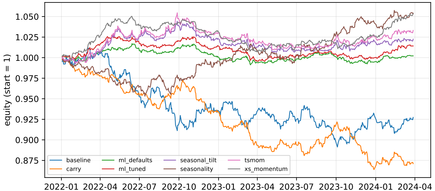
Out-of-sample 2022-2024Q1 — net equity, 2 bps/side, 10% vol target
