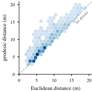
(b) Spatial difficulty
