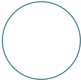
CUBIC CIRCLE: EXACT SPLINES
