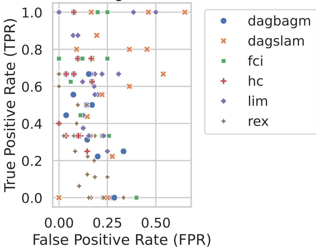
TPR vs FPR across algorithms and datasets
