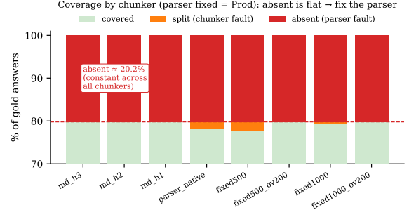
Figure 2: The coverage diagnostic (C2): with the parser fixed (Prod) and the chunker varied, each gold answer is covered , split (a chunker fault, recoverable with overlap), or absent (a parser fault, unrecoverable by chunking). The absent rate is \approx 20.2\% and essentially constant across all eight chunkers, while split is at most 2.3% (§4.2)—chunking cannot close a gap the parser already lost, so the fix must be parser-side.
