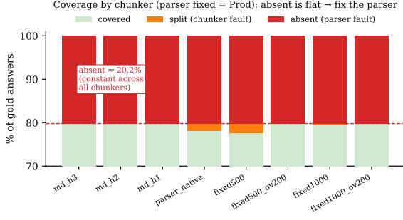
Figure 1: The coverage diagnostic (C2): with the parser fixed (Prod) and the chunker varied, each gold answer is covered , split (a chunker fault, recoverable with overlap), or absent (a parser fault, unrecoverable by chunking). The absent rate is \approx 20.2\% and essentially constant across all eight chunkers, while split is at most 2.3% (§4.2)—chunking cannot close a gap the parser already lost, so the fix must be parser-side.
