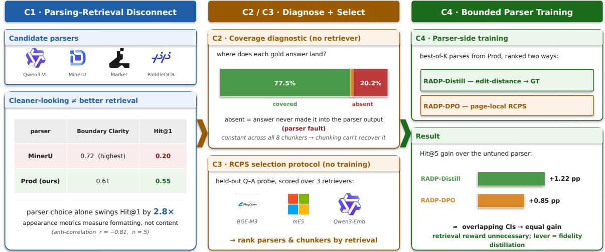
Figure 1: Overview. (C1) Selecting a document parser by appearance (Boundary Clarity) rather than retrieval is a trap: MinerU has the highest Boundary Clarity yet the lowest Hit@1, and parser choice alone swings Hit@1 by 2.8\times ( r = -0.81 at n = 5 is illustrative; the robust signal is the mechanism). (C2) A retriever-free coverage diagnostic localises the gap to the parser—20.2% of answers are absent from the parser output, constant across all eight chunkers. (C3) RCPS selects parsers and chunkers by retrieval over a held-out Q-A probe and three retrievers, with no training. (C4) Parser-side training is a bounded lever: best-of- K fidelity distillation (RADP-Distill) matches the retrieval-reward variant (RADP-DPO) (+1.22 vs +0.85 pp Hit@5, overlapping CIs), so the retrieval reward is unnecessary.
