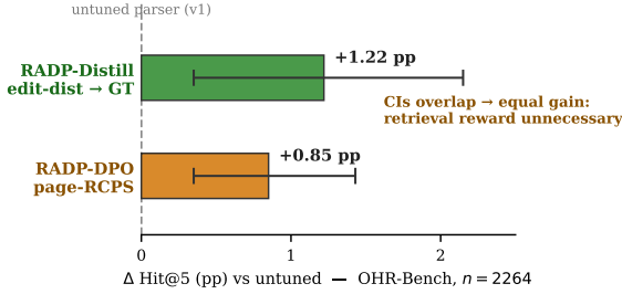
Figure 5: Parser-side training (C4): OHR-Bench Hit@5 gain over the untuned parser for the two ways of ranking best-of-K candidates. Ranking by edit-distance to ground truth (RADP-Distill, +1.22 pp) and by page-local RCPS (RADP-DPO, +0.85 pp) are both significant and their confidence intervals overlap—a statistically indistinguishable gain. The retrieval reward is therefore unnecessary; the deployable lever is fidelity distillation (3-retriever avg, n=2264 ).
