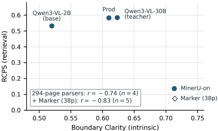
(a) MinerU-on diagnostic: BC can misrank
