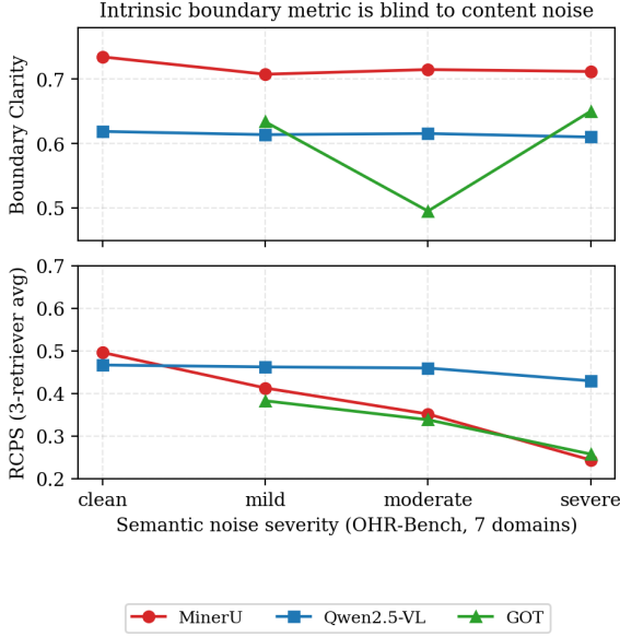
Figure 2: OHR-Bench seven-domain noise-family curves. Top: Boundary Clarity does not track noise severity—flat for MinerU and Qwen2.5-VL, non-monotone for GOT. Bottom: RCPS collapses for MinerU and GOT, and falls more gently for the noise-robust Qwen2.5-VL. The intrinsic metric does not perceive the content corruption retrieval depends on.
