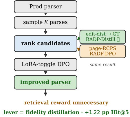
Figure 4: Parser-side training (C4), a best-of-K pipeline. Ranking candidates by edit-distance to ground truth (RADP-Distill) reproduces ranking by page-local RCPS (RADP-DPO), so the retrieval reward is unnecessary—the deployable lever is fidelity distillation (+1.22 pp Hit@5, OHR-Bench).
