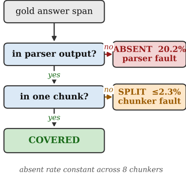
Figure 1: The coverage diagnostic (C2): each gold answer is covered , split (a chunker fault, recoverable with overlap), or absent (a parser fault, unrecoverable by chunking). On Prod, 20.2% are absent and at most 2.3% split, the absent rate constant across all eight chunkers (§4.2)—so the gap is a parser problem.
