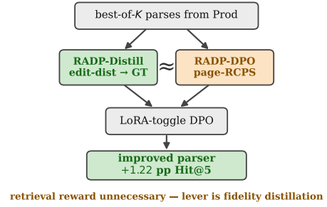
Figure 4: Parser-side training (C4), a best-of-K pipeline. Ranking candidates by edit-distance to ground truth (RADP-Distill) reproduces ranking by page-local RCPS (RADP-DPO), so the retrieval reward is unnecessary—the deployable lever is fidelity distillation (+1.22 pp Hit@5, OHR-Bench).
