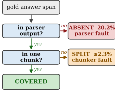
Figure 1: The coverage diagnostic (C2): each gold answer is covered , split (a chunker fault, recoverable with overlap), or absent (a parser fault, unrecoverable by chunking). On Prod, 20.2% are absent and at most 2.3% split, the absent rate constant across all eight chunkers (§4.2)—so the gap is a parser problem.
