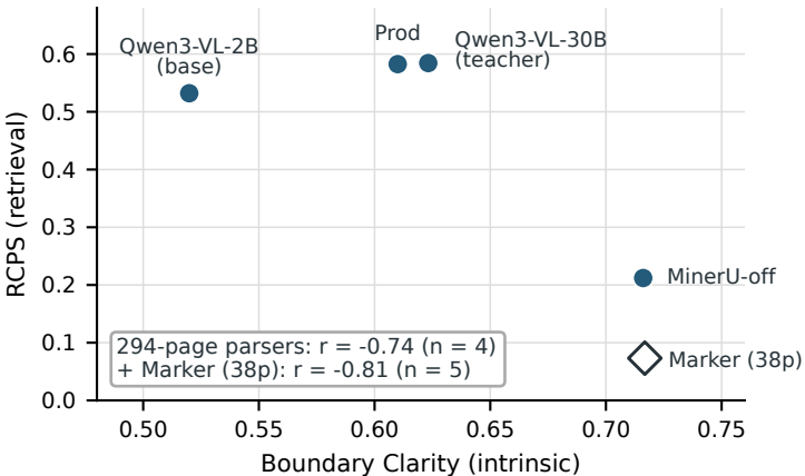
(a) MinerU-off diagnostic: BC can misrank
