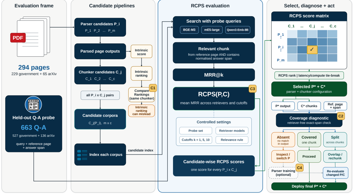
Figure 1: RCPS workflow . A held-out Q–A probe evaluates parser–chunker candidates. Intrinsic and RCPS parser rankings can disagree (C1); coverage separates spans absent from parser output from those split across chunk boundaries (C2); RCPS ranks candidates across fixed retrievers and cutoffs (C3); and parser training is reserved for unresolved parser-side failures before changed configurations are re-evaluated (C4).
