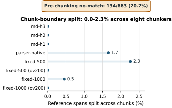
Figure 3: Coverage with Prod fixed (294 pages, 663 Q–A; no retriever). Absence is measured before chunking and stays 20.2%; changing the chunker affects only splitting, which reaches at most 2.3%.
