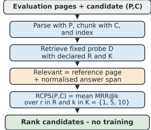
Figure 2: RCPS compares candidates on the same held-out Q-A probe. It averages standard MRR over declared retrievers and cutoffs; a hit must come from the reference page and contain the normalised reference answer. Use a singleton retriever set when deployment is fixed, or a declared set when it is undecided. Evaluation itself requires no training.
