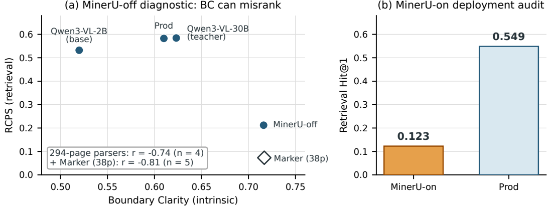
Figure 4: In this candidate pool, higher Boundary Clarity (BC) does not imply better retrieval. (a) Among four 294-page parsers with defined BC, the correlation with RCPS is r = -0.74 ( n = 4 ); adding Marker’s partial 38-page output gives r = -0.81 ( n = 5 ). MinerU-off is used in this diagnostic. (b) In the separate MinerU-on deployment comparison, Prod exceeds MinerU-on Hit@1 by 42.6 points (0.549 vs. 0.123; 4.47\times ).
