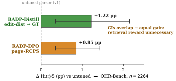
Figure 4: Parser-side training (C4): OHR-Bench Hit@5 gain over the untuned parser for the two ways of ranking best-of- K candidates. Ranking by edit-distance to ground truth (RADP-Distill, +1.22 pp) and by page-local RCPS (RADP-DPO, +0.85 pp) are both significant and their confidence intervals overlap—a statistically indistinguishable gain. The retrieval reward is therefore unnecessary; the deployable lever is fidelity distillation (3-retriever avg, n=2264 ).
