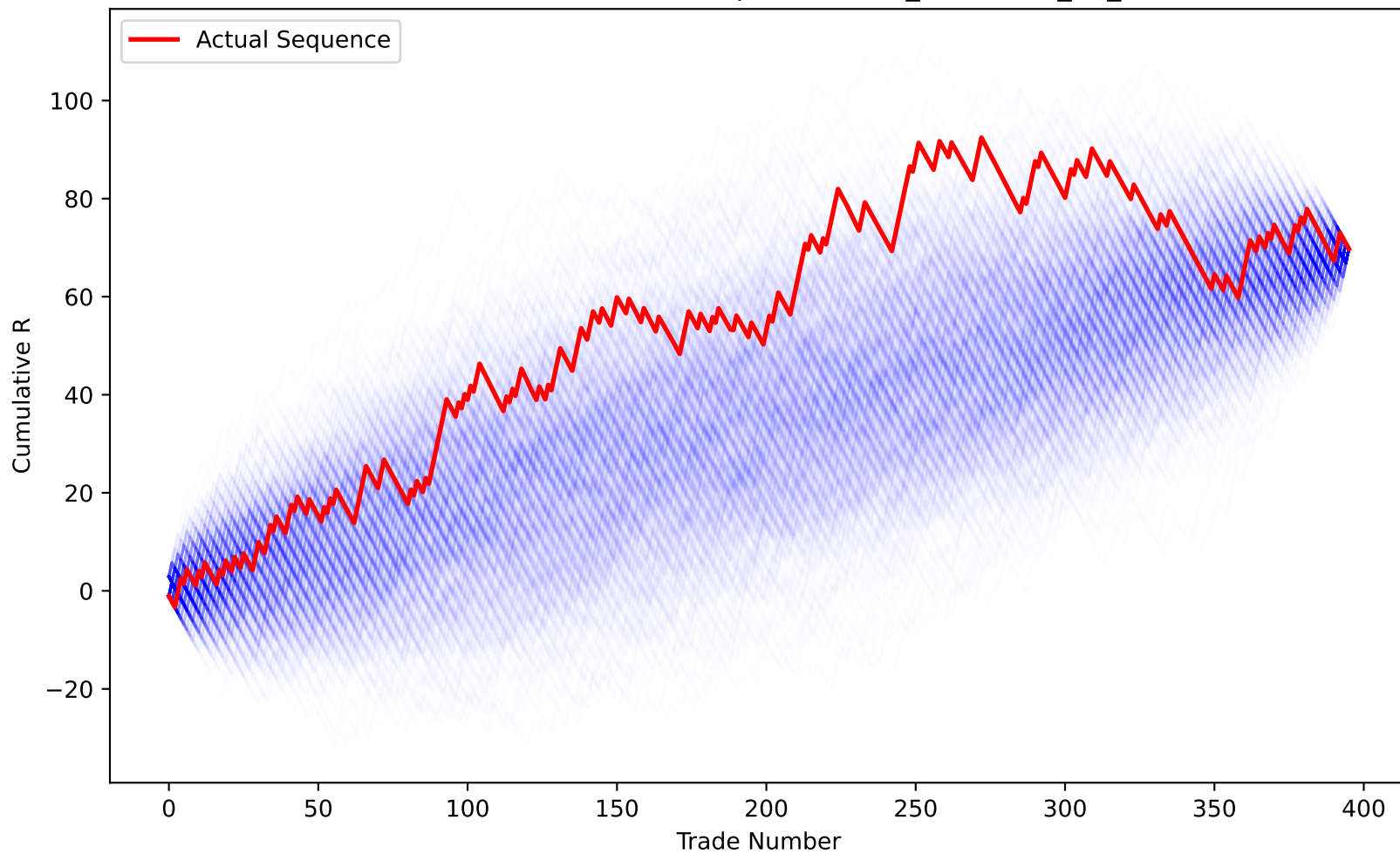
Monte Carlo Shuffle (1000 paths) - ATR_Percentile_10_20
