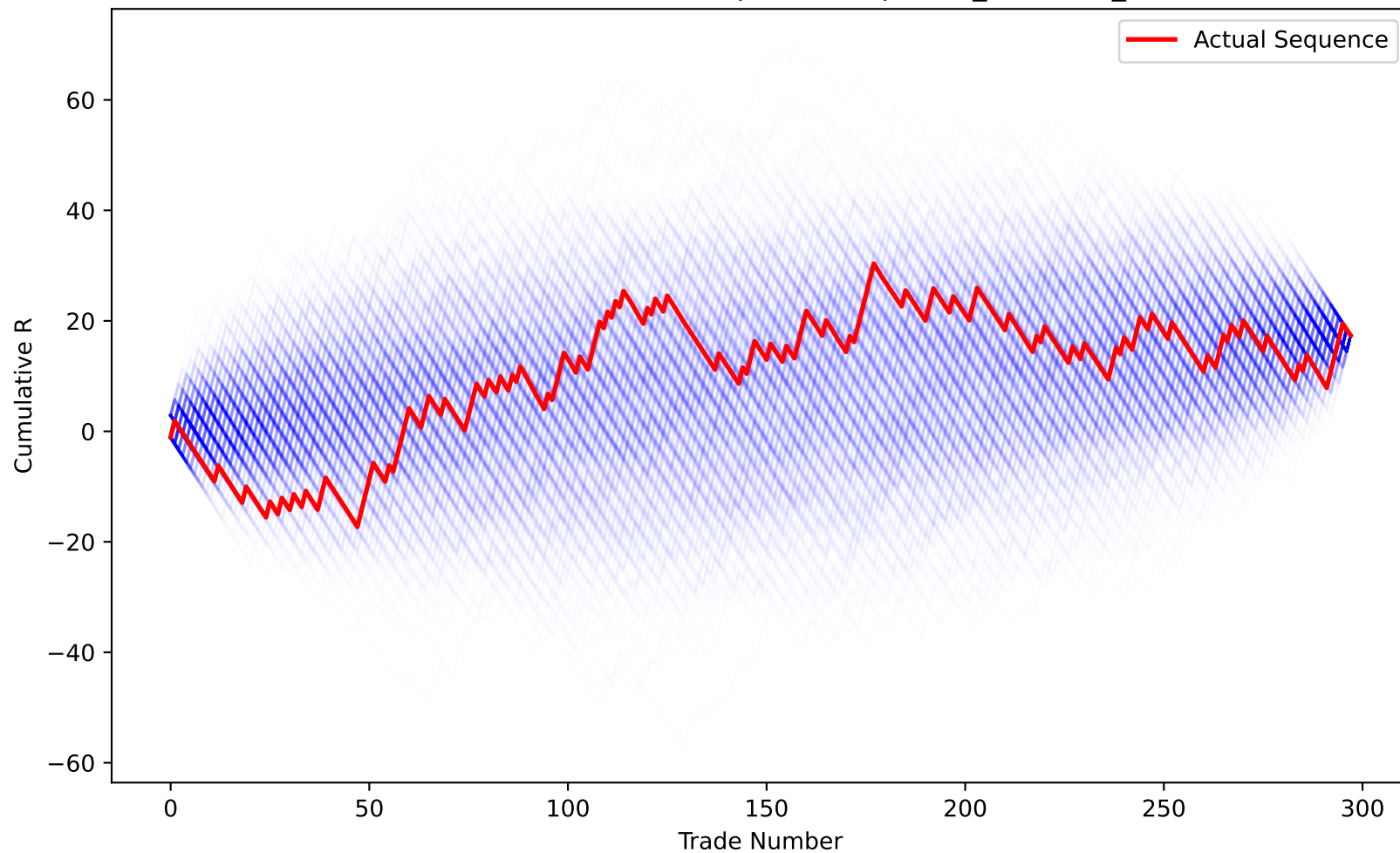
Monte Carlo Shuffle (1000 paths) - Squeeze_Breakout_L3
