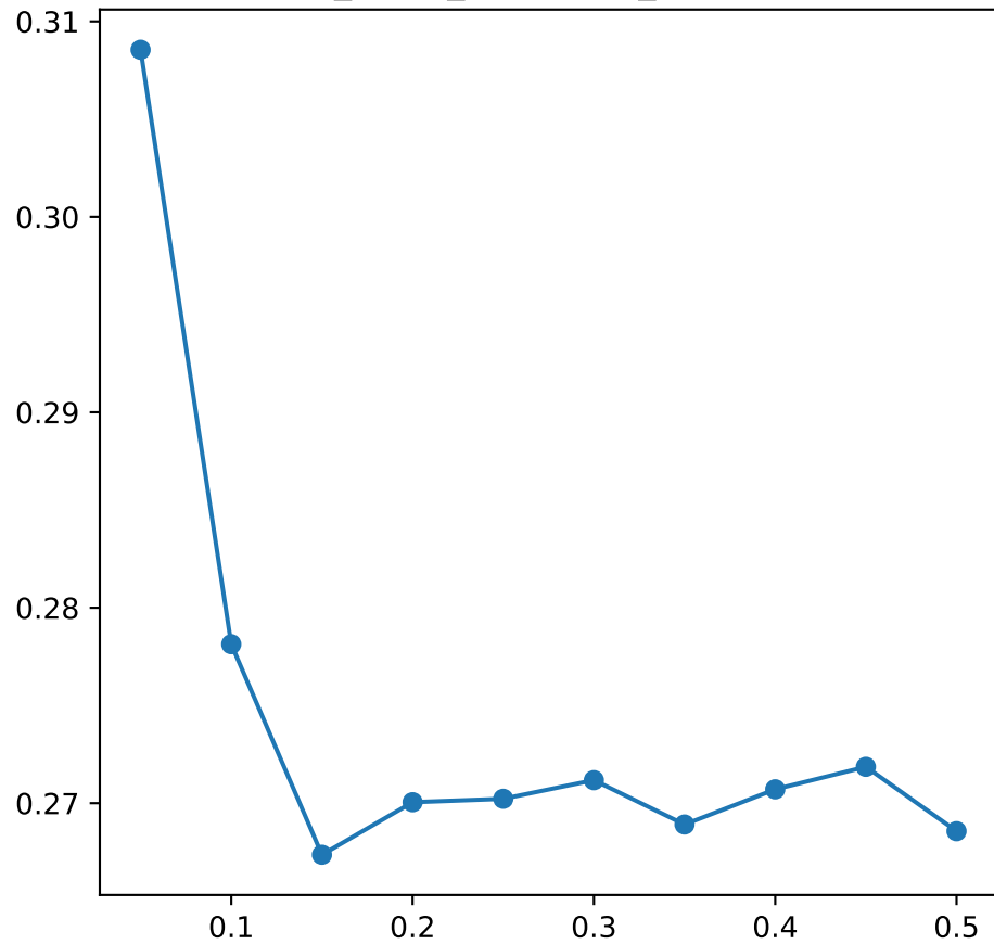
donchian_width_percentile_100 -> P(3ATR)
