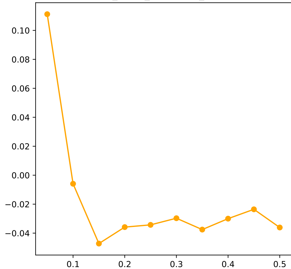
donchian_width_percentile_100 -> EES
