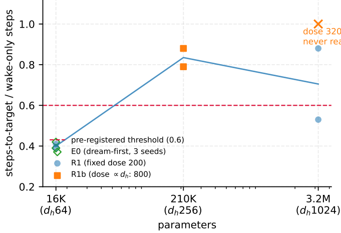
Figure 1: Dream advantage is capacity-bound. Steps-to-target ratio (lower is better; pre-registered threshold 0.6 dashed). At 16K parameters dream-first reaches wake-only’s final accuracy with \sim 40\% of the interactions (five independent runs across two platforms). At 210K/3.2M the advantage fades; scaling the dream budget with width (R1b) does not restore it, and at the largest scale the highest dose never reaches the target.
