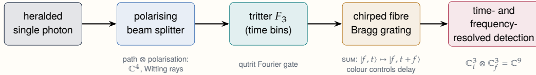
Figure 31. One photon, two qutrits. The controlled-add (sum) gate between the frequency and time qutrits has been demonstrated with a single passive element, a chirped fibre Bragg grating, at basis fidelity 0.92 \pm 0.01 [19].
