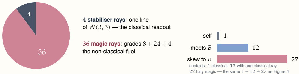
Figure 32. The machine’s quantum resource is the geometry itself: remove one line and every remaining point is a magic state.
