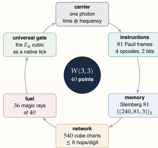
Figure 30. The Holonet stack. Every layer is a structure of W(3,3) read as engineering: the Pauli frames are the 81 points of \mathbb{F}_3^4 , the memory is the Steinberg module, the network is the geometry's atlas of cube charts, the fuel is its set of magic states, and the universal gate is the E_6 cubic of Section 5.
