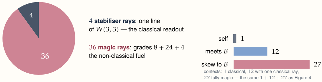
Figure 32. The machine’s quantum resource is the geometry itself: remove one line and every remaining point is a magic state.
