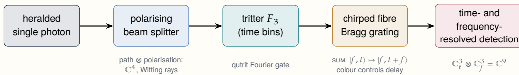
Figure 34. One photon, two qutrits. The controlled-add (SUM) gate between the frequency and time qutrits has been demonstrated with a single passive element, a chirped fibre Bragg grating, at basis fidelity 0.92 \pm 0.01 [25].
